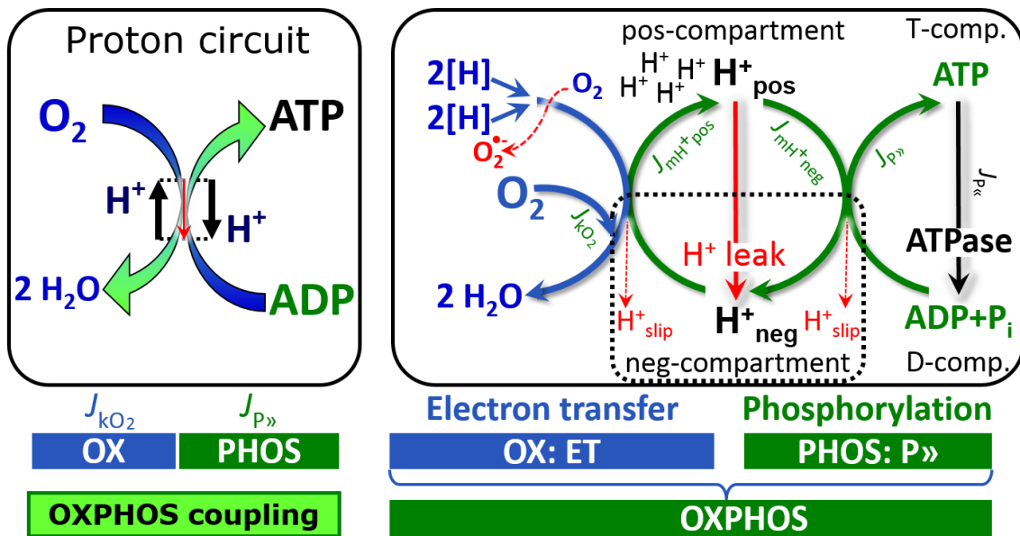
Fig. 2. The proton circuit and coupling in oxidative phosphorylation (OXPHOS). 2[H] indicates the reduced hydrogen equivalents of fuel substrates of the catabolic reaction k with oxygen. O_2 flux, J_{kO_2} , through the catabolic ET-pathway, is coupled to flux through the phosphorylation-pathway of ADP to ATP , J_{P\gg} . The proton pumps of the ET-pathway drive proton flux into the positive (pos) compartment, J_{mH^+pos} , generating the output protonmotive force (motive, subscript m ). F-ATPase is coupled to inward proton current into the negative (neg) compartment, J_{mH^+neg} , to phosphorylate ADP+P_i to ATP . The system defined by the boundaries (full black line) is not a black box, but is analysed as a compartmental system. The negative compartment (neg-compartment, enclosed by the dotted line) is the matrix space, separated by the mtIM from the positive compartment (pos-compartment). ADP+P_i and ATP are the substrate- and product-compartments (scalar ADP and ATP compartments, D-comp. and T-comp.), respectively. At steady-state proton turnover, J_{\infty H^+} , and ATP turnover, J_{\infty P} ,
