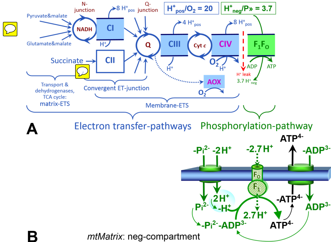
Fig. 1. The oxidative phosphorylation (OXPHOS) system. (A) The mitochondrial electron transfer system (ETS) is fuelled by diffusion and transport of substrates across the mtOM and mtIM and consists of the matrix-ETS and membrane-ETS. ET-pathways are coupled to the phosphorylation-pathway. ET-pathways converge at the N-junction and Q-junction. Additional arrows indicate electron entry into the Q-junction through electron transferring flavoprotein, glycerophosphate dehydrogenase, dihydro-orotate dehydrogenase, choline dehydrogenase, and sulfide-ubiquinone oxidoreductase. The dotted arrow indicates the branched pathway of oxygen consumption by alternative quinol oxidase (AOX). The H^+_{pos}/O_2 ratio is the outward proton flux from the matrix space to the positively (pos) charged compartment, divided by catabolic O_2 flux in the NADH-pathway. The H^+_{neg}/P \gg ratio is the inward proton flux from the inter-membrane space to the negatively (neg) charged matrix space, divided by the flux of phosphorylation of ADP to ATP (Eq. 1). These are not fixed stoichiometries due to ion leaks and proton slip. (B) Phosphorylation-pathway catalyzed by the proton pump F 1 F 0 -ATPase (F-ATPase, ATP synthase), adenine nucleotide translocase, and inorganic phosphate transporter. The H^+_{neg}/P \gg stoichiometry is the sum of the coupling stoichiometry in the F-ATPase reaction (-2.7 H^+_{pos} from the positive intermembrane space, 2.7 H^+_{neg} to the matrix, i.e., the negative compartment) and the proton balance in the translocation of ADP 2- , ATP 3- and P i 2- . Modified from (A) Lemieux et al. (2017) and (B) Gnaiger (2014).
