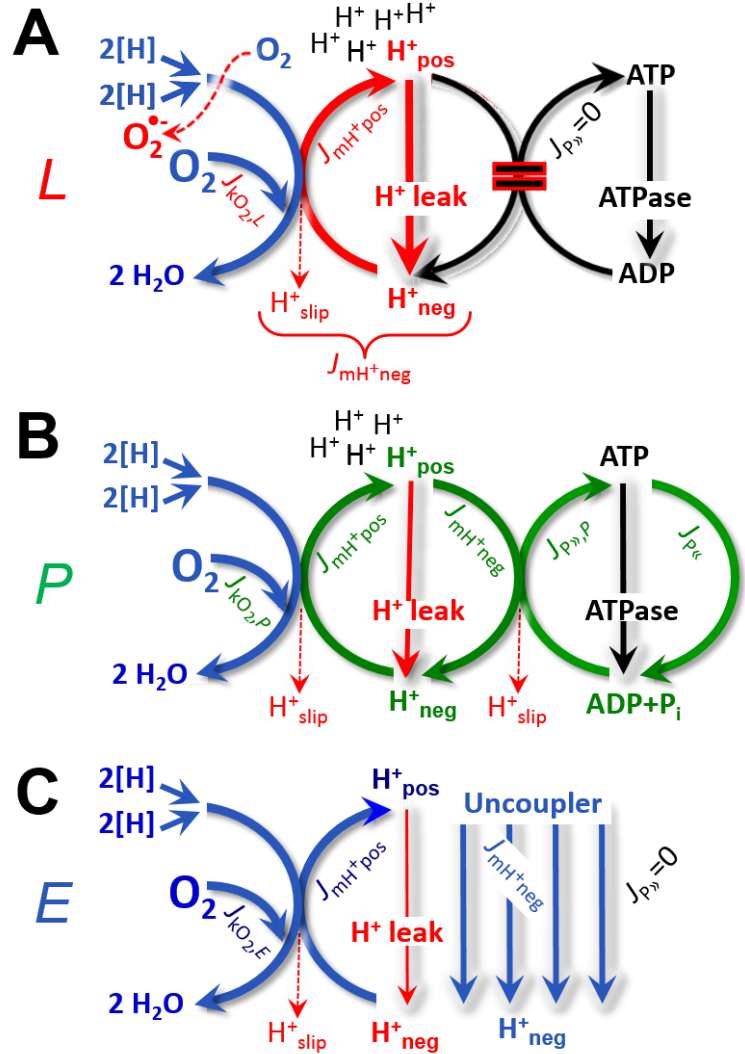
Fig. 5. Respiratory coupling states. A: LEAK-state and rate, L: Phosphorylation is arrested, J_{P\gg} = 0 , and catabolic O_2 flux, J_{kO_2,L} , is controlled mainly by the proton leak, J_{mH^+neg,L} , at maximum protonmotive force (Fig. 3). B: OXPHOS-state and rate, P: Phosphorylation, J_{P\gg} , is stimulated by kinetically-saturating [ADP] and [P_i] , and is supported by a high protonmotive force. O_2 flux, J_{kO_2,P} , is well-coupled at a P\gg/O_2 ratio of J_{P\gg,P}/J_{kO_2,P} . C: ET-state and rate, E: Noncoupled respiration, J_{kO_2,E} , is maximum at optimum exogenous uncoupler concentration and phosphorylation is zero, J_{P\gg} = 0 . See also Fig. 2.
