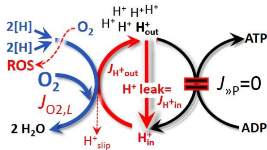
Fig. 3. LEAK state when phosphorylation is arrested, J_{\gg P} = 0 , and LEAK oxygen flux, J_{O_2,L} , is controlled mainly by the proton leak, which equals J_{H^+,in} , at maximum \Delta p_{mt} (compare Fig. 1).
