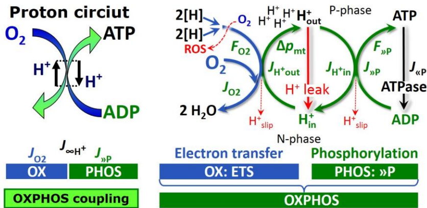
Fig. 1. The proton circuit and coupling in oxidative phosphorylation (OXPHOS). Oxygen flux, J_{O_2} , is coupled to the phosphorylation of ADP to ATP, J_{\gg P} , by the proton pumps of the electron transfer system (ETS) pushing the outwards proton flux, J_{H^+out} . The ATP synthase is driven by the protonmotive force, \Delta p_{mt} , and inwards proton flux, J_{H^+in} , to phosphorylate ADP to ATP. 2[H] indicates the reduced hydrogen equivalents of fuel substrates providing the chemical input force or molar Gibbs energy, F_{O_2} [kJ/mol O_2 ], of the reaction with oxygen, typically in the range of -460 to -480 kJ/mol. The output force is given by the phosphorylation potential, F_{\gg P} [kJ/mol ADP phosphorylated to ATP], which varies in vivo in the range of about 48 to 62 kJ/mol under physiological conditions. Proton turnover, J_{\infty H^+} , and ATP turnover, J_{\gg P} , proceed in the steady state at constant \Delta p_{mt} , when J_{\infty H^+} = J_{H^+out} = J_{H^+in} , and at constant phosphorylation potential, F_{\gg P} , when J_{\gg P} = J_{\ll P} = J_{\ll P} . J_{\gg P}/J_{O_2} is two times the 'P/O' ( \gg P/O ) ratio of classical bioenergetics. The effective J_{\gg P}/J_{O_2} ratio is diminished by (i) the proton leak across the inner mt-membrane from low pH in the positive P-phase to the negative N-phase, (ii) cycling of other cations, (iii) proton slip of the proton pumps, and (iv) electron leak generating reactive oxygen species, ROS. Modified after Gnaiger (2014).
