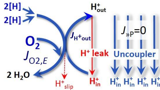
Fig. 5. ETS state when noncoupled respiration, J_{O_2,E} , is maximum at optimum exogenous uncoupler concentration and phosphorylation is zero, J_{>>P}=0 (compare Fig. 1).
