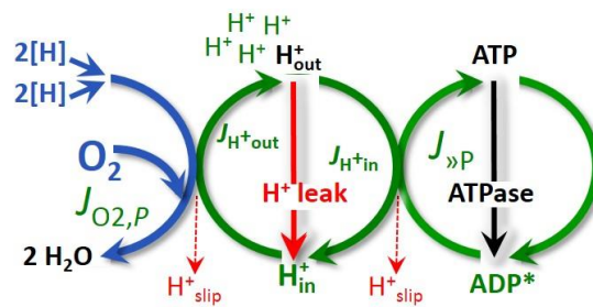
Fig. 4. OXPHOS state when phosphorylation, J_{\gg P} , is supported by a high \Delta p_{mt} , is stimulated by saturating [ADP]^* and [Pi]^* , and oxygen flux, J_{O2,P} , is highly coupled at a maximum \gg P/O_2 ratio, J_{\gg P}/J_{O2,P} (compare Fig. 1).
