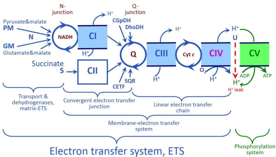
Fig. 2. The mitochondrial respiratory system. In oxidative phosphorylation the electron transfer system (A) is coupled to the phosphorylation system (B). Modified after (A) Lemieux et al (2017) and (B) Gnaiger (2014).
