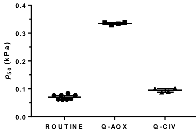
Figure 2. p_{50} values obtained for different metabolic pathways in C. reinhardtii . O_2 kinetic experiments were run in presence of the cytochrome c oxidase inhibitor potassium cyanide (AOX group) or the alternative oxidase inhibitor salicylhydroxamic acid (CIV group). The data represents n=8 technical replicates, N=2 , median \pm IR.
