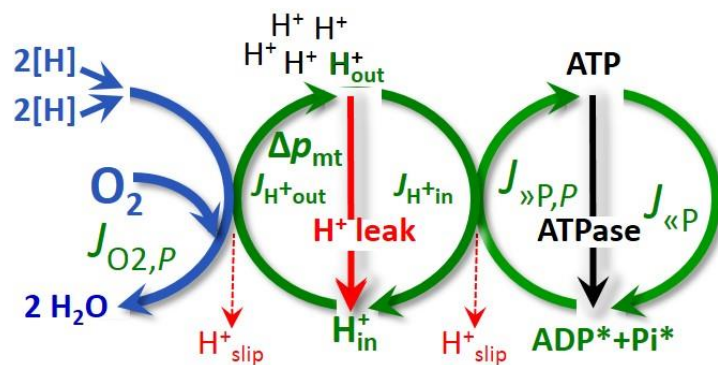
Fig. 3. OXPHOS state: Phosphorylation, J_{»P} , is supported by a high \Delta p_{mt} , is stimulated by kinetically saturating [ADP]* and inorganic phosphate, [P i ]*. O 2 flux, J_{O_2,P} , is highly coupled at a maximum »P/O_2 ratio, J_{»P,P}/J_{O_2,P} (See also Fig. 2).
