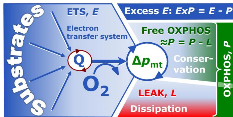
Fig. 6. Four-compartmental model of oxidative phosphorylation with respiratory states (ETS, OXPPOS, LEAK) and corresponding rates ( E , P , L ).
