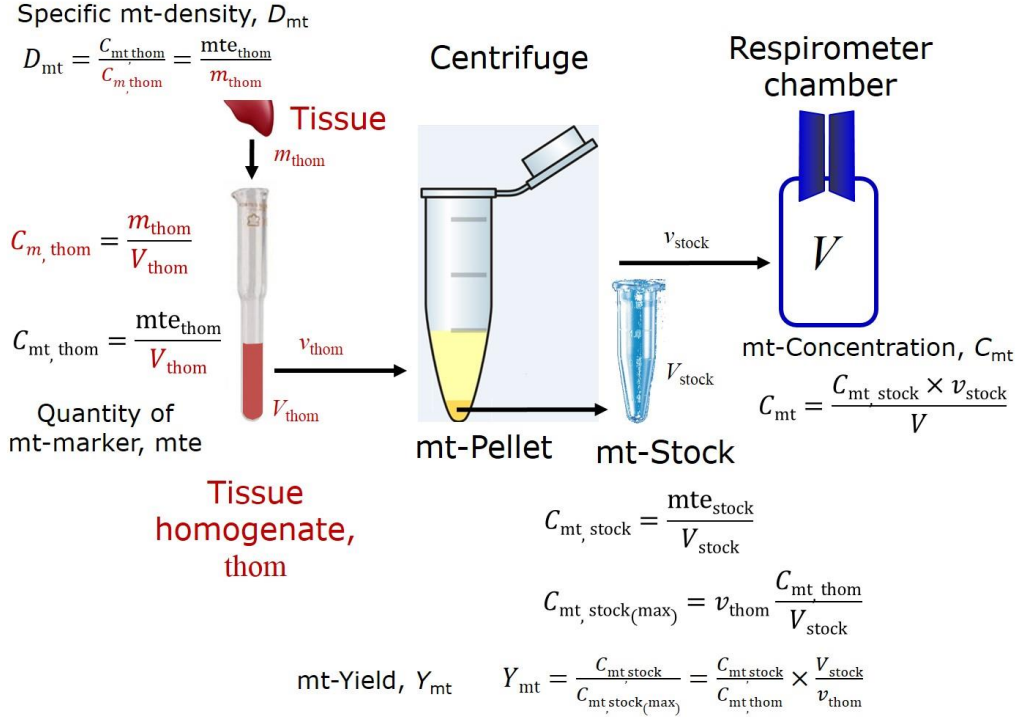
Fig. 8. Mitochondrial yield, Y_{mt} , in preparation of isolated mitochondria. See Table 4 for explanation of symbols.
