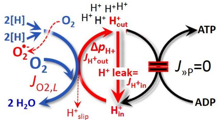
Fig. 5. LEAK state: Phosphorylation is arrested, J_{\gg P}=0 , and oxygen flux, J_{O_2, L} , is controlled mainly by the proton leak, which equals J_{H^+ in} , at maximum \Delta p_{H^+} (See also Fig. 2).
