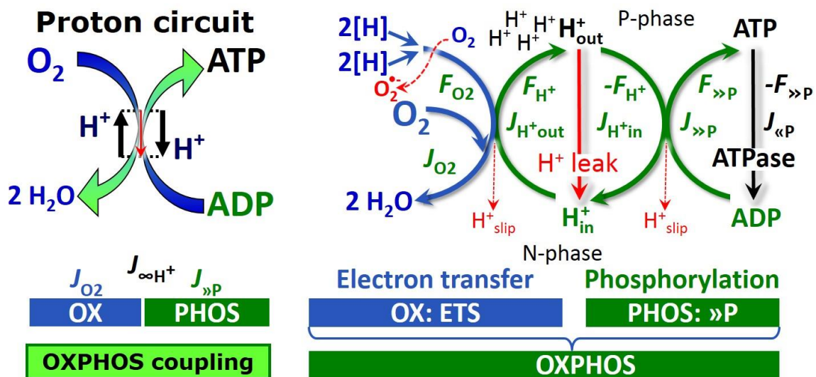
Fig. 2. The proton circuit and coupling in oxidative phosphorylation (OXPHOS). Oxygen flux, J_{O_2} , is coupled to the phosphorylation of ADP to ATP, J_{»P} , by the proton pumps of the
