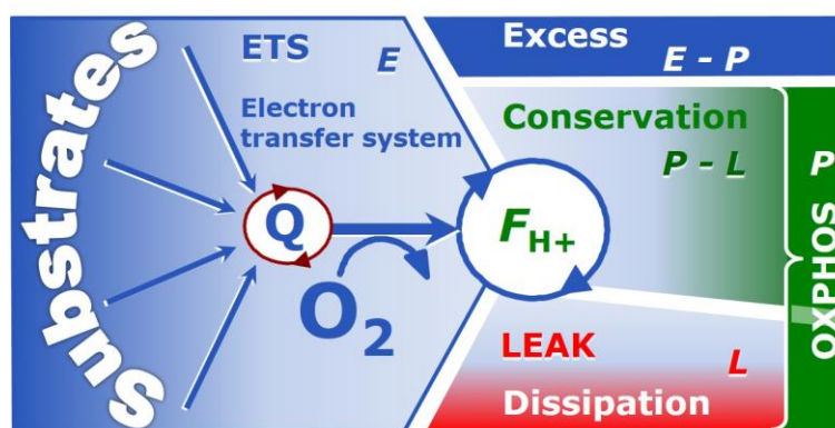
Fig. 6. Four-compartmental model of oxidative phosphorylation. Respiratory states (ETS, OXPHOS, LEAK) and corresponding rates ( E , P , L ) are connected by the protonmotive force, F_{H+} . Electron transfer system
