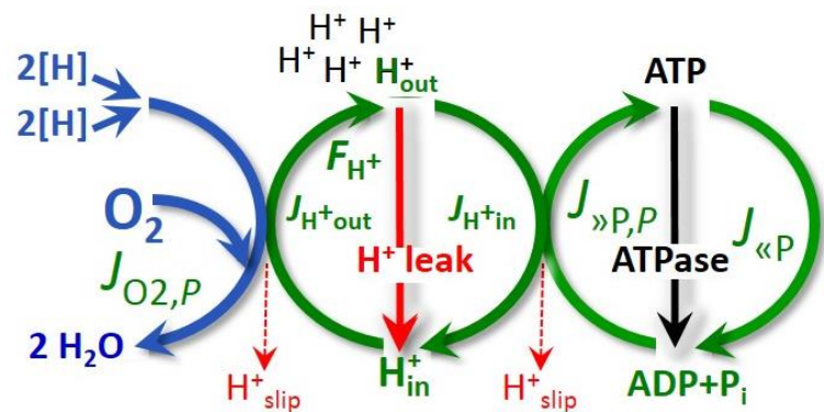
Fig. 3. OXPHOS state: Phosphorylation, J_{\gg P} , is stimulated by kinetically saturating [ADP] and inorganic phosphate, [Pi], and is supported by a high protonmotive force, F_{H^+} . O_2 flux, J_{O_2,P} , is highly coupled at a maximum \gg P/O_2 ratio, J_{\gg P,P}/J_{O_2,P} (See also Fig. 2).
